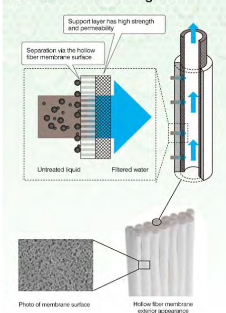
Membrane Filtration Diagram
